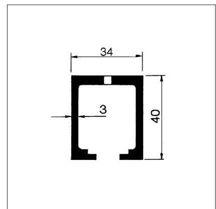
Ceiling profile detail.
