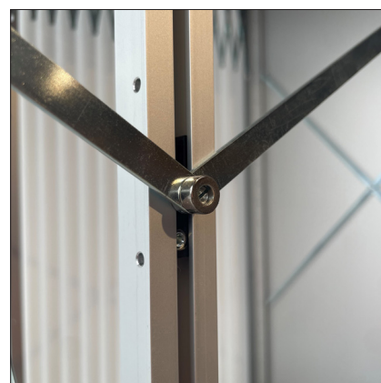
The crosses are connected at the back with magnets. This means the shelf can be easily rearranged
